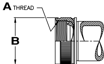
Style A, R & S INTERFACE PER SAE AS85049 FIGURE 4 O'RING NOT REQUIRED / SUPPLIED
